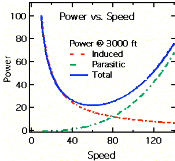
Fig 11 Power requirements versus speed.
