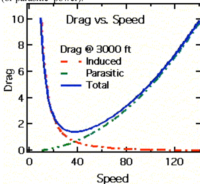
Fig 12 Drag versus speed.
