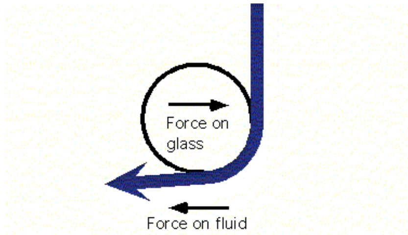
Fig 8 Coanda effect.
