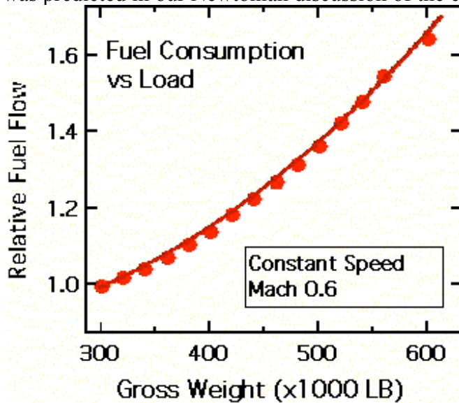
Fig 13 Fuel consumption versus load for a large transport airplane traveling at a constant speed.
